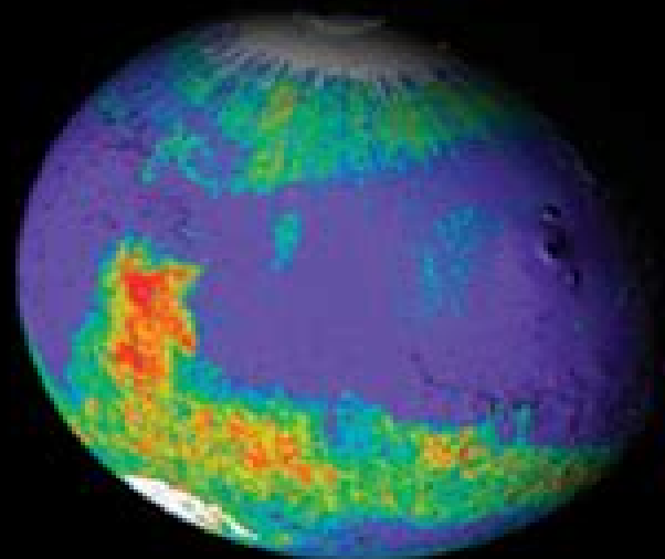
Mineral Abundance
