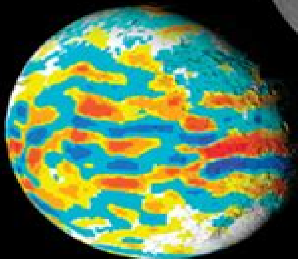
Remanant Magnetism
