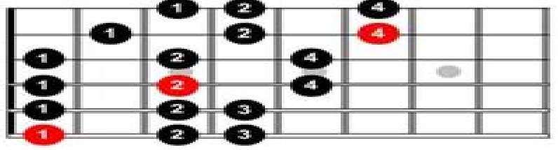
Aeolian (natural minor)
