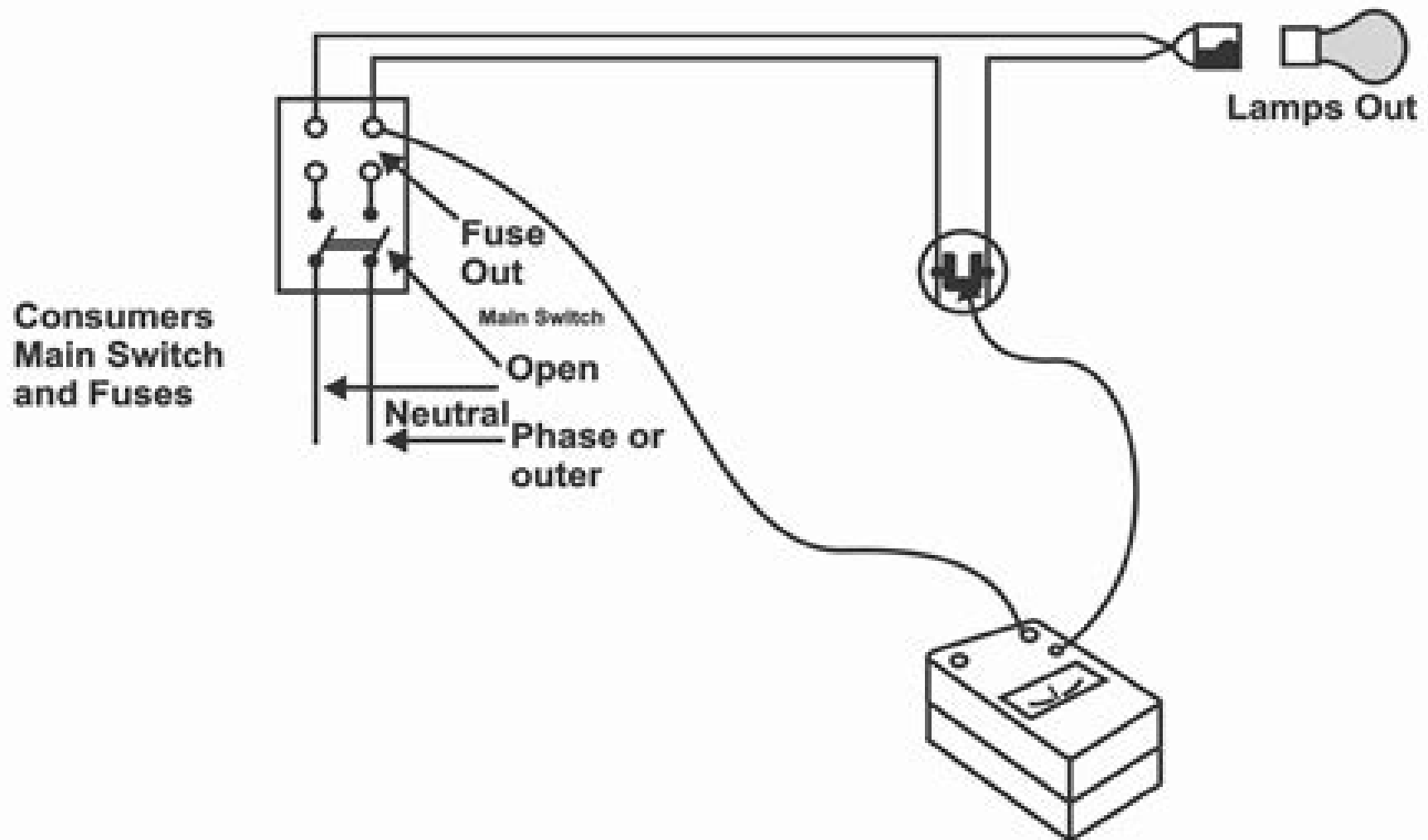
Fig 1.17 Testing for polarity of switch with circuit dead.
