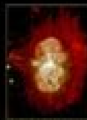
Red Dwarf Star A red dwarf star is a small, dimly glowing star that is the most common type of star in the universe. It is much smaller and cooler than our Sun, and can live for trillions of years.
