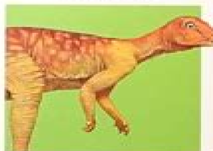
Zephyrosaurus
