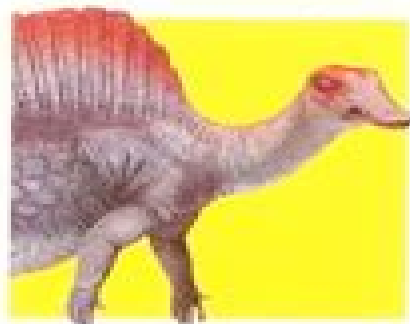
Ouranosaurus
