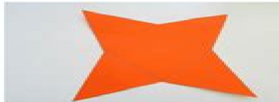
SQUARE-BASED PYRAMID
