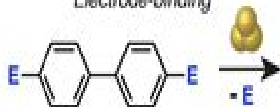
Electrode-binding
