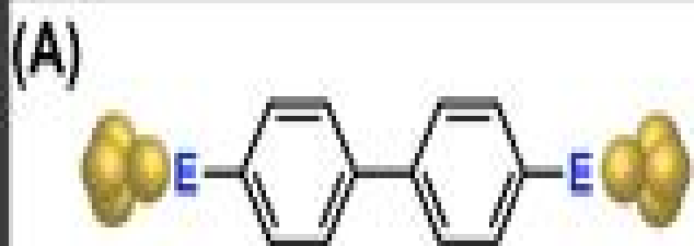
Electrode-binding
