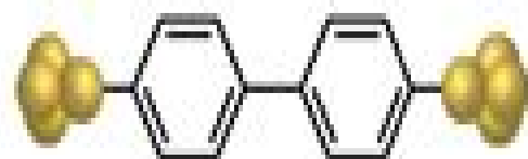
Electrode-reactive
