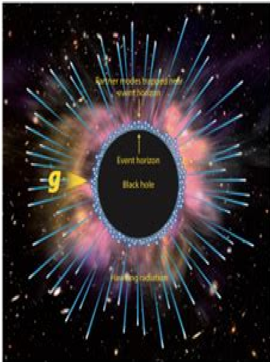
Black hole Hawking evaporation
