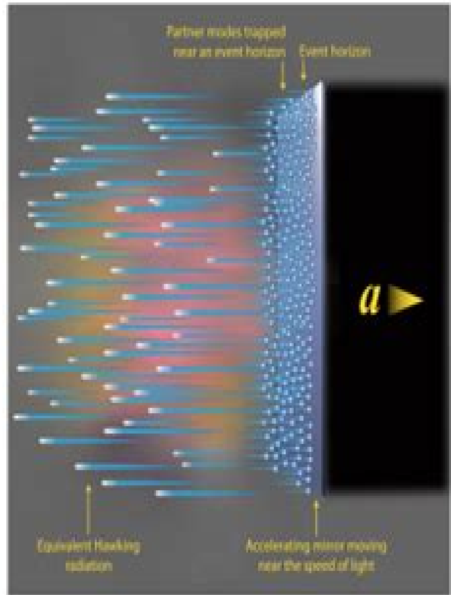
Accelerating mirror as an analog black hole
