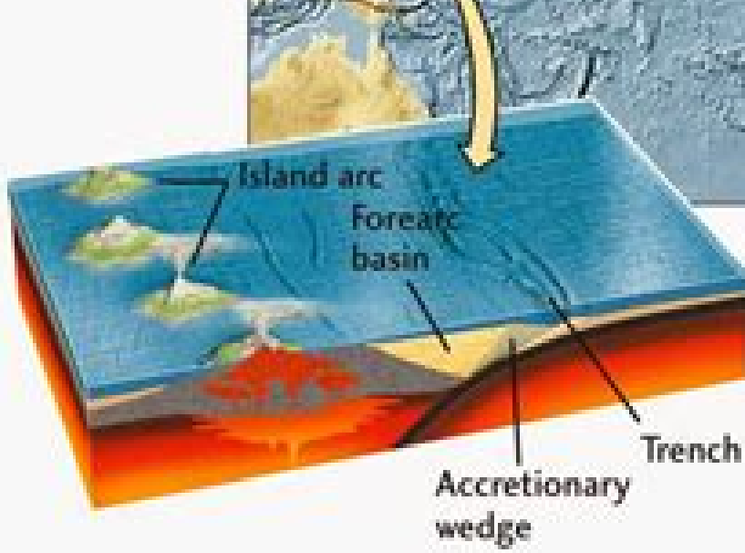
(b) Active margin of the Marianas type
