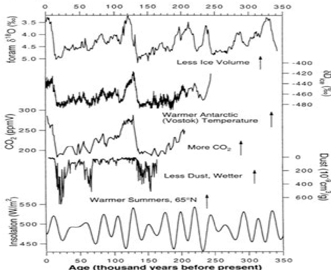
FIG. 4. Selected ice core records for the last 350 kyr. Data from refs. 34–37.
