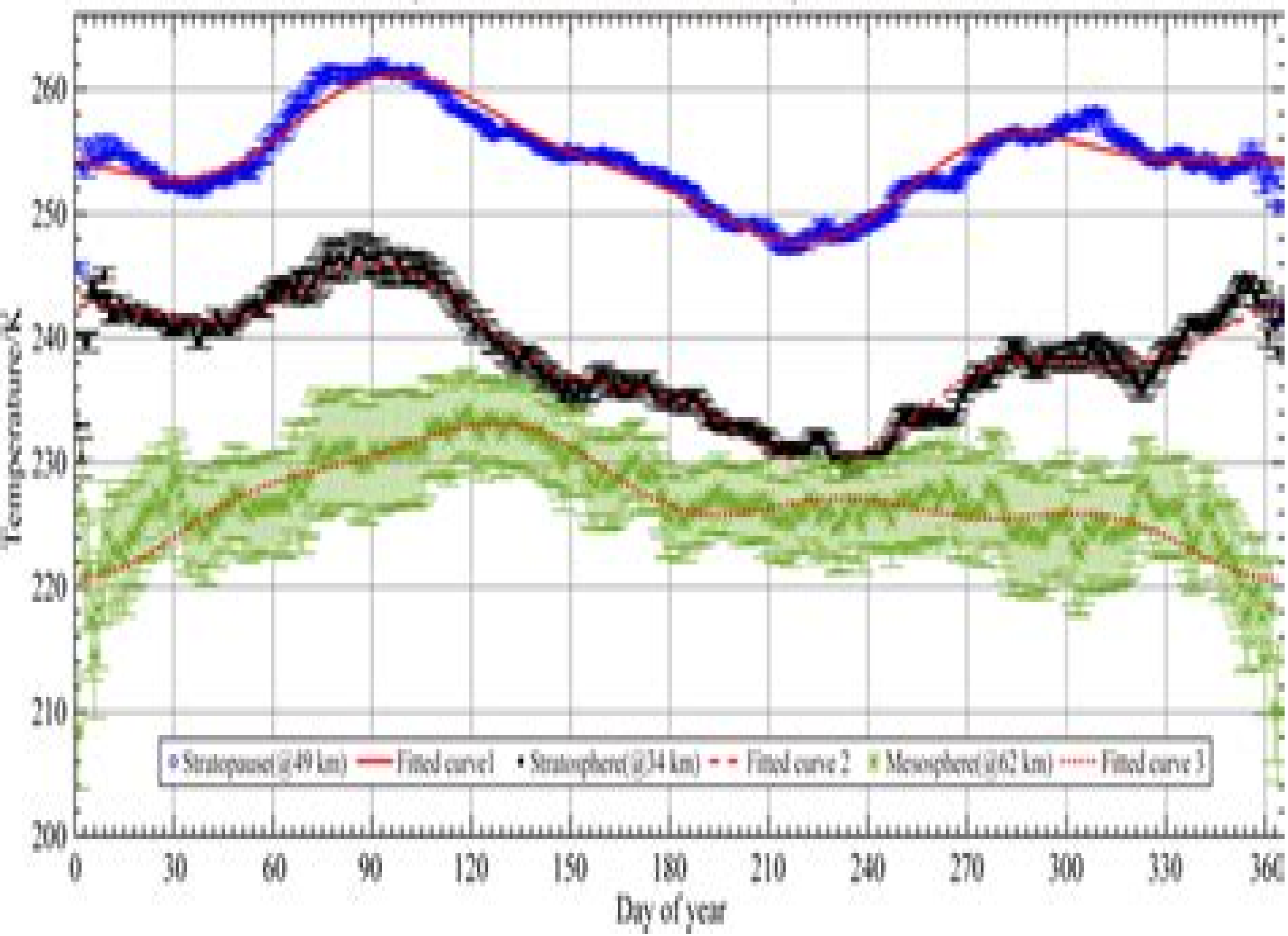
Temperature oscillations in the middle atmosphere over Haikou
