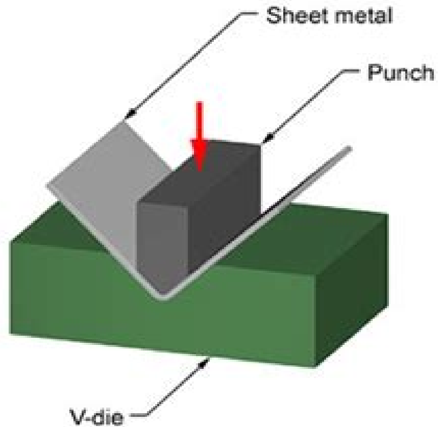
Bottoming
