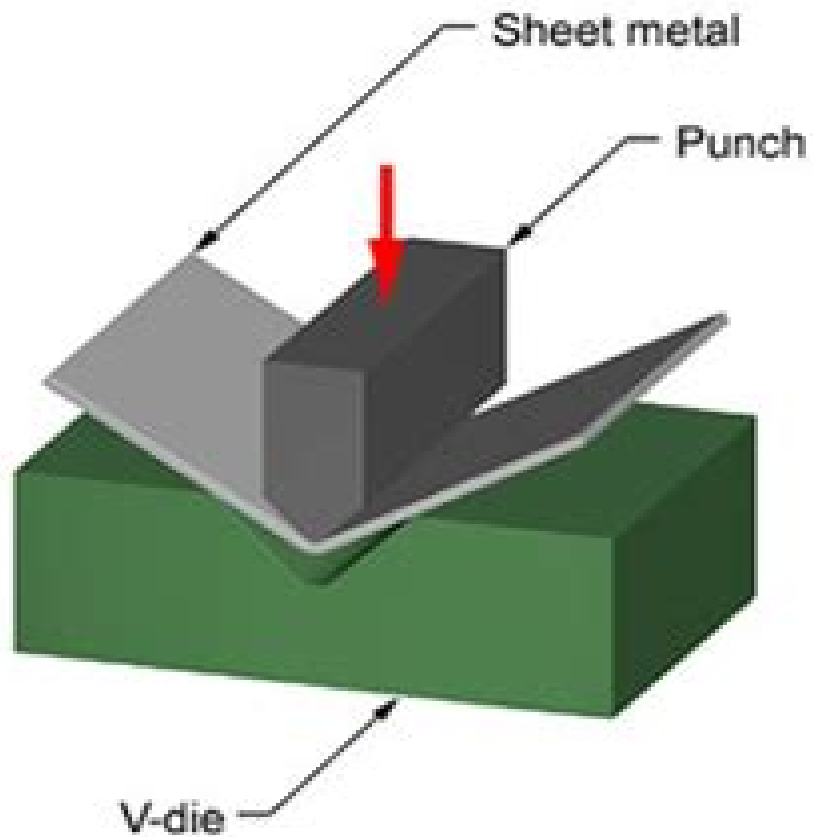
Air Bending
