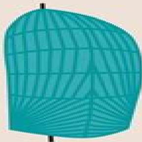
SYMMETRICAL SPINNAKER
