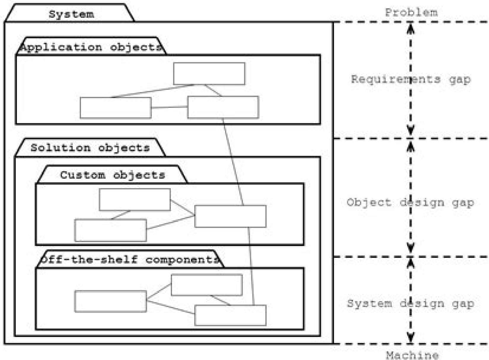
Figure 7-1. Object design closes the gap between application objects identified during requirements and off-the-shelf components selected during system design (stylized UML class diagram).
