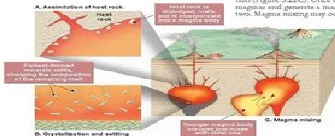
FIGURE 3.22 This illustration shows three ways that the composition of a magma body may be altered: A. Assimilation of host rock; B. Crystallization and settling (magmatic differentiation); and C. Magma mixing.
