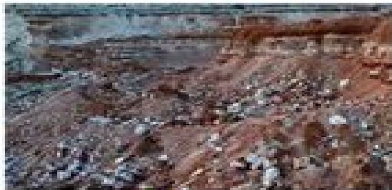
Antimony-tungsten deposits after the magmatic period
