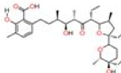
Lasalocid A C_{36}H_{54}O_8 MW 590.79
