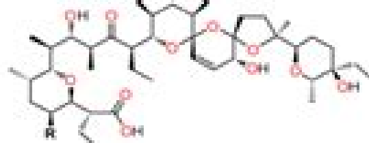
Salinomycin R=H C_{42}H_{70}O_{11} MW 751.00 Narasin R=CH_3 C_{43}H_{72}O_{11} MW 765.03
