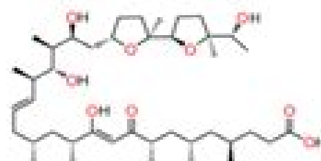
Ionomycin C_{43}H_{72}O_9 MW 709.00
