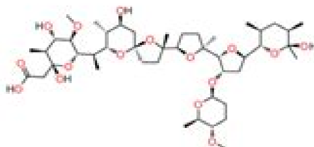
Semduramycin C_{46}H_{76}O_{16} MW 873.08
