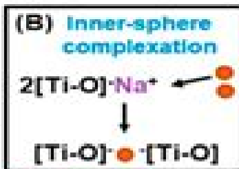
Interaction mechanism of Ba^{2+}/Sr^{2+} by MXene J. Environ. Manage. 2020, 256, 109940
