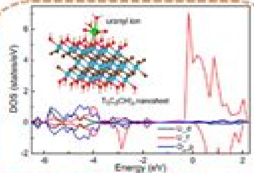
MXenes applied for U(VI) removal J. Hazard. Mater. 2016, 308, 482-489
