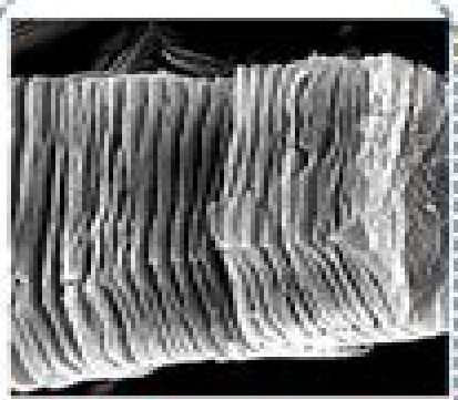
Ti_3AlCN after HF treatment ACS Nano, 2012, 4, 1322-1331
