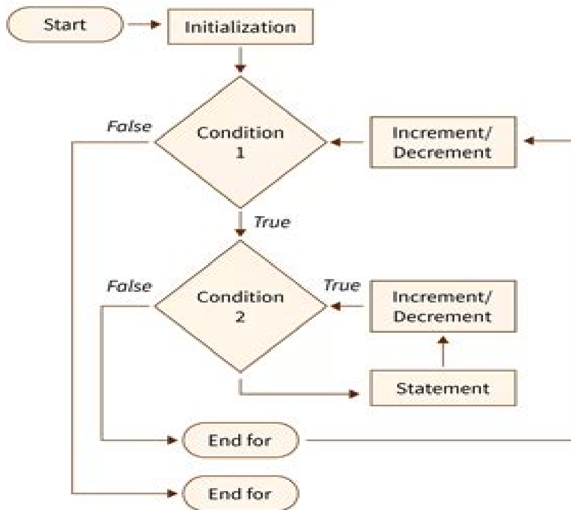
Flow chart for nested do-while loop
