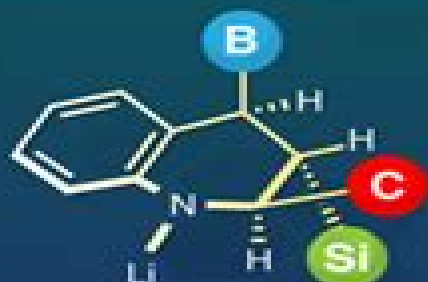
Dearomative triple elementalization
