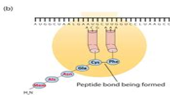
(b) An activated tRNA, which has the anticodon AAA, binds to the ribosome next to the previous bound tRNA and interacts with the mRNA molecule though base-pairing of the codon and anticodon. The amino acid Phe is being incorporated into the polypeptide chain by the formation of a peptide linkage between the carboxyl group of Cys and the amino acid group of the Phe. This reaction is catalyzed by the enzyme peptidyl transferase, a component of the ribosome.
