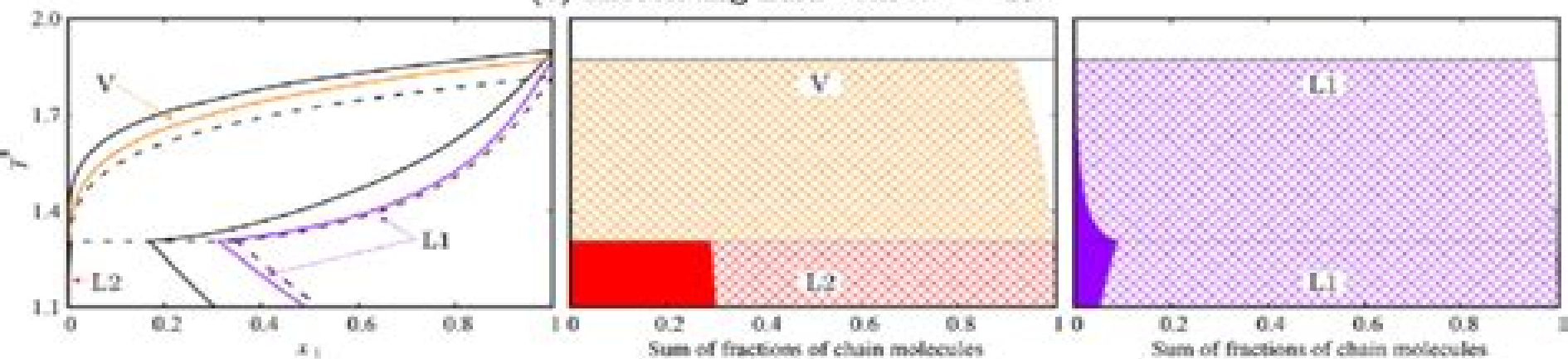
(c) Associating fluid with W^* = 100 .
