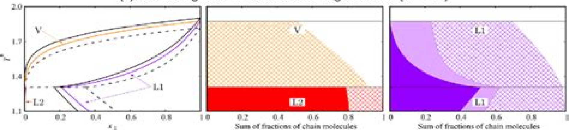
(b) Associating fluid with W^* = 10 .
