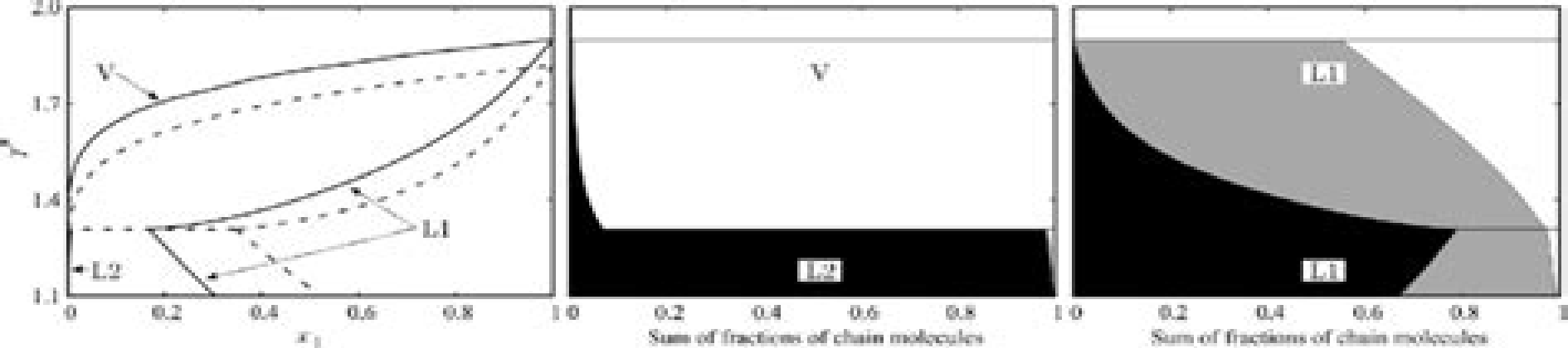
(a) Associating fluid in the absence of ring formation ( W^* = 0 ).
