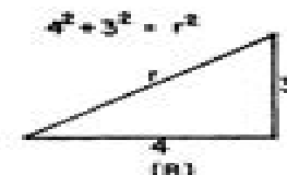
Figure 19-2.—The Pythagorean Theorem.
