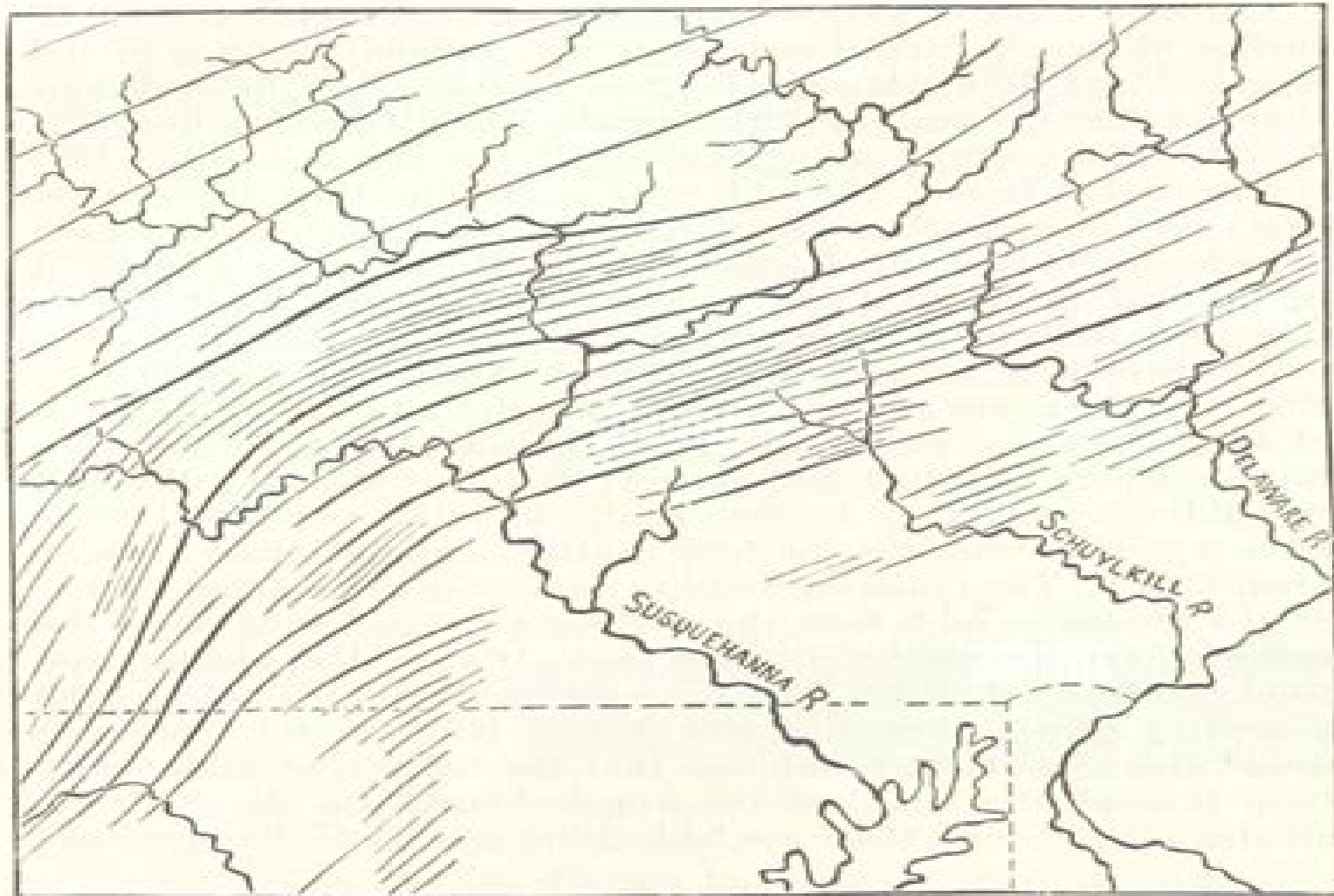
Map of Pennsylvania, showing the positions of the axes of the folds in the strata.
