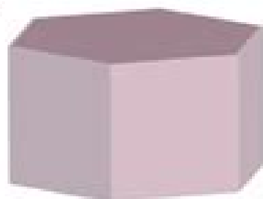
Hexagonal prism
