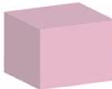
Cube
