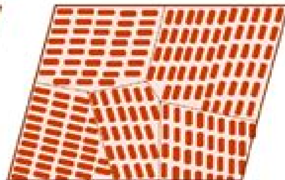
Polycrystalline
