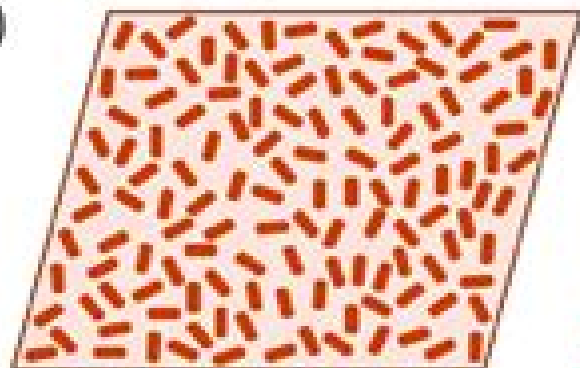
Amorphous
