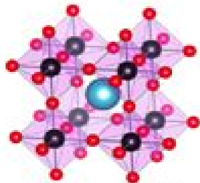
Inorganic perovskite
