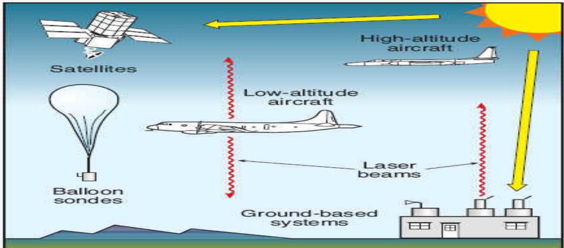
Figure Q5-1. Ozone measurements. Ozone is measured throughout the atmosphere with instruments on the ground, aircraft, high-altitude balloons, and satellites. Some instruments measure ozone locally in sampled air and others measure ozone remotely some distance away from the instrument. Instruments use optical techniques, with the Sun and lasers as light sources; detect the microwave emissions from ozone; or use chemical reactions that are unique to ozone. At many locations over the globe, regular measurements are made to monitor total ozone amounts and their variations over time.
