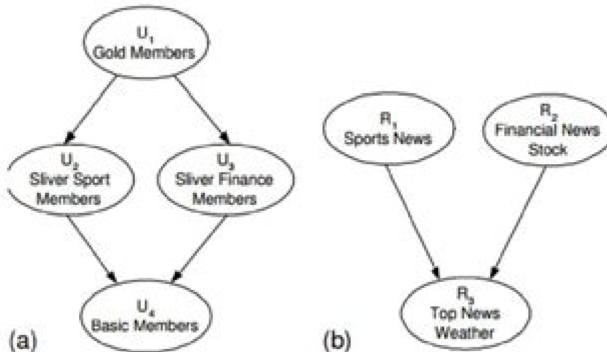
Figure 1: (a)Membership group DAG, (b) resource group DAG
