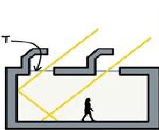
ROOF MONITOR
