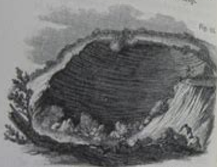
Channel formed by the earthquake of 1811 near Havana, in Cuba.
