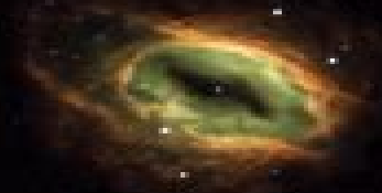
Eye of Sauron Nebula (M 1-42)
