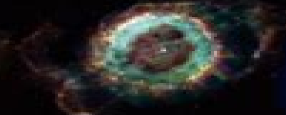
Eye of Sauron Nebula (M 1-42)
