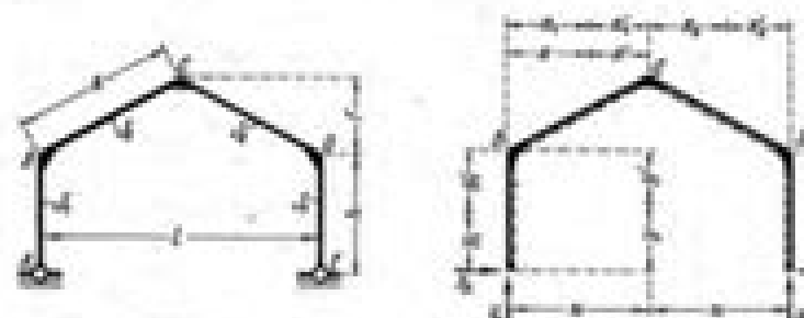
Shape of Frame Dimensions and Notations
