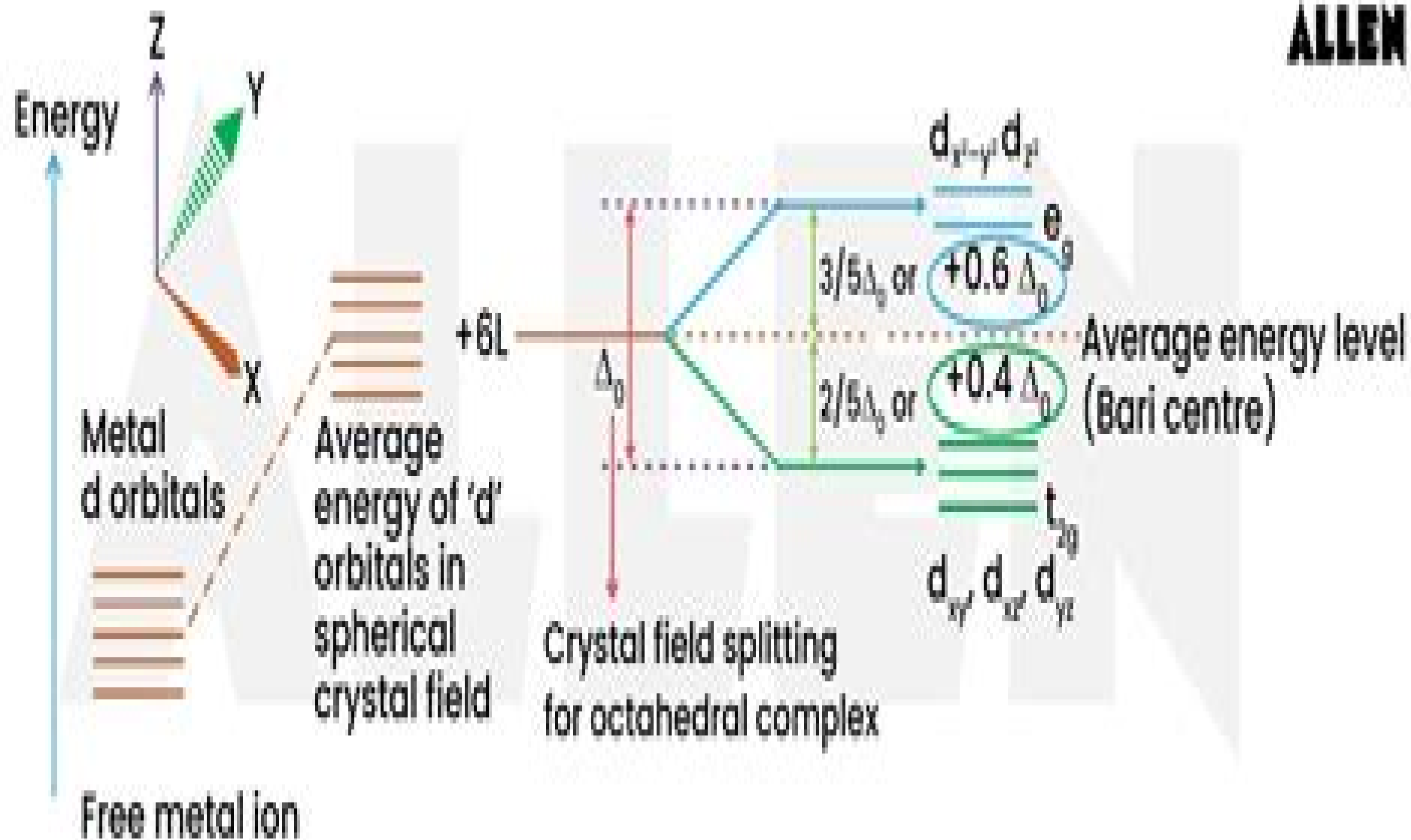
Crystal field splitting in octahedral complex
