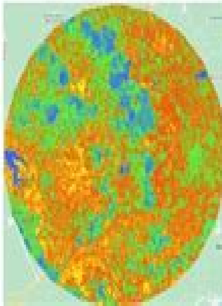
Rock alternation
