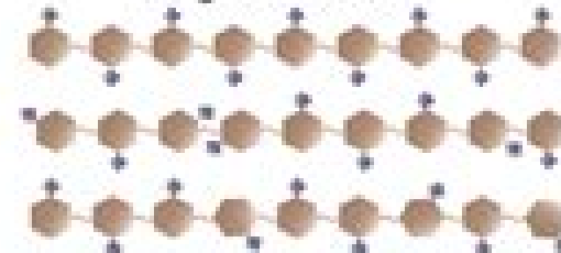
Segment sequences
