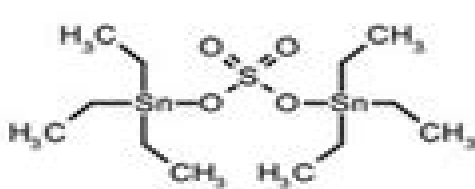
Triethyltin sulfate
