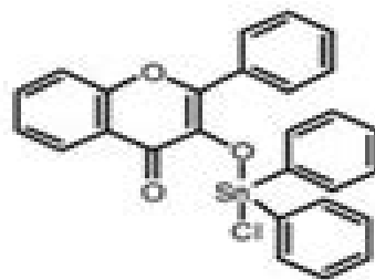
Diphenyltin 3- hydroxy- flavone chloride
