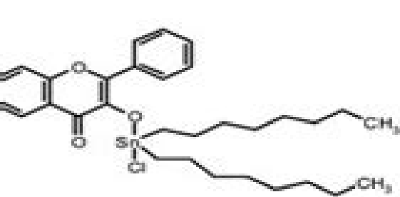
Dioctyltin 3- hydroxy- flavone chloride
