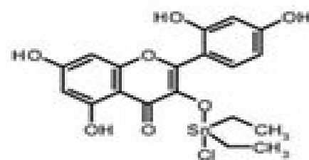
Dimethyltin 3- hydroxy- flavone chloride
