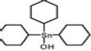
cyclohexyltin hydroxide
