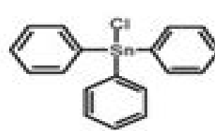
Triphenyltin chloride
