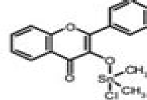
Dimethyltin 3- hydroxy- flavone chloride
