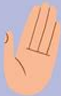
Assertiveness
