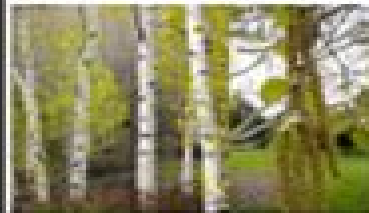
state tree
