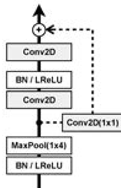
(b) ResNet block
