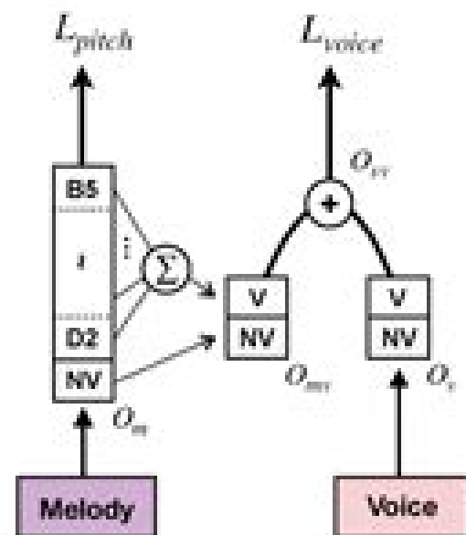
(c) Joint melody loss
