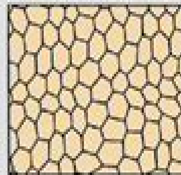
Fully recrystallized
