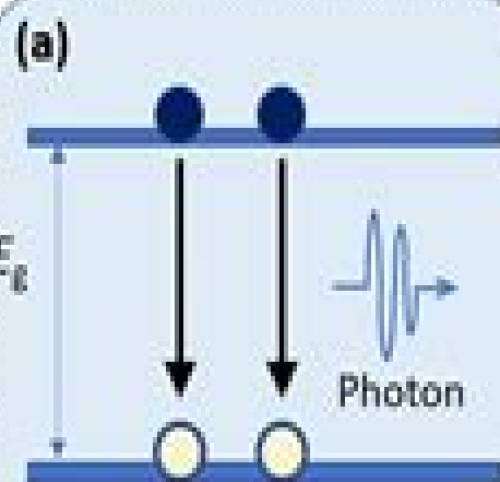
Radiative recombination
