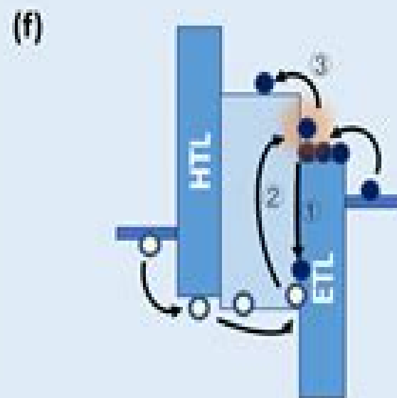
Interface-induced Auger recombination
