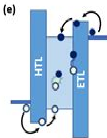
Non-radiative recombination in the emitter layer and at the interface
