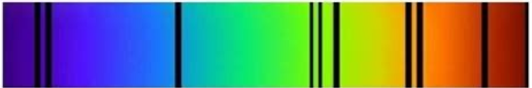
Blueshifted spectrum
