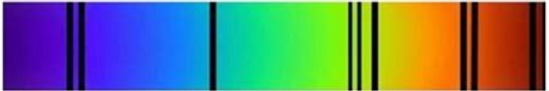
Redshifted spectrum
