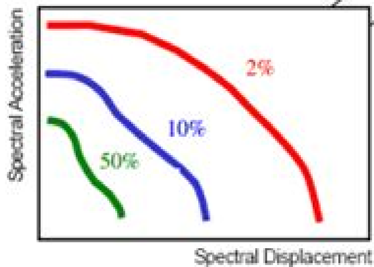
Ground Motion Demand Curves
