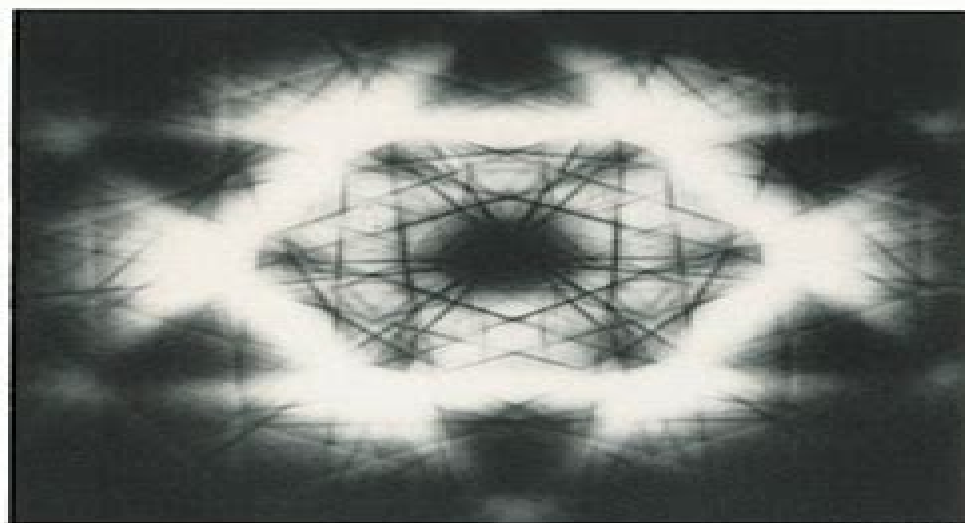
[0001] convergent beam electron diffraction pattern of \alpha -Al 2 O 3
