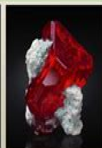
Oxides - Cuprite
