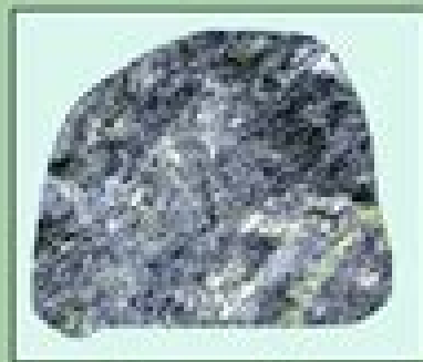
Blue schist
