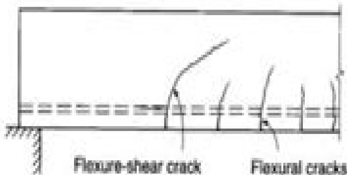
(b) Flexure-shear cracking
