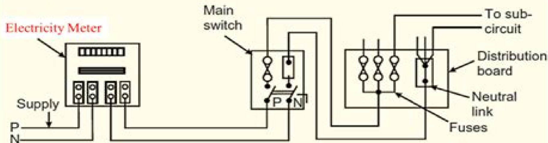
Fig. 1: Connections of electricity meter to measure electrical energy of a domestic consumer
