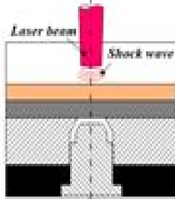
(j) Laser shock micro clinching
