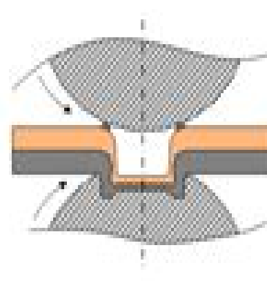
(k) Roller clinching
