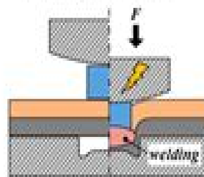
(c) Hole clinching
