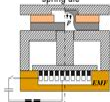
(i) Hole clinching with EMF
