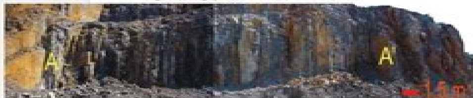
Figure 3. Field views of K-bentonites at limestone quarries excavated in Yılanı formation
