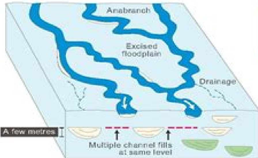
Anastomosing River
