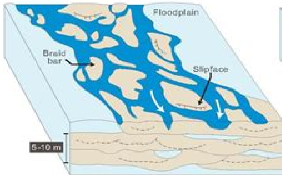
Braided River
