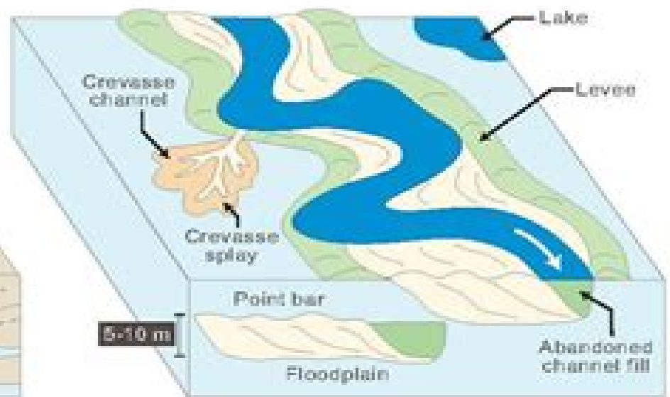
Meandering River
