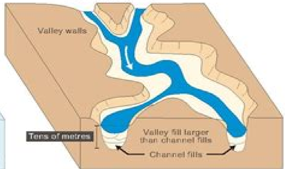
Valley System
